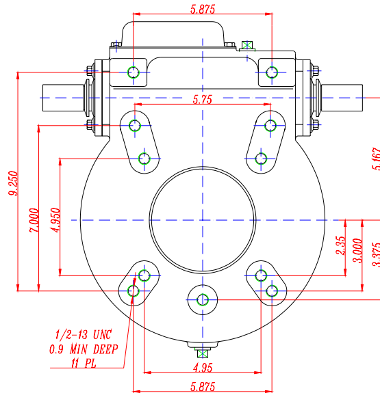
REAR VIEW TYPICAL
