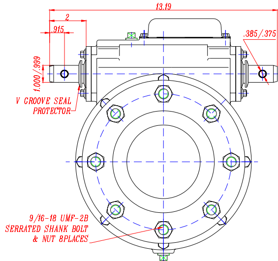
FRONT VIEW TYPICAL
